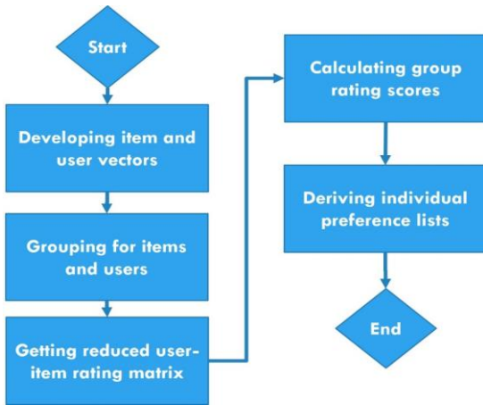
Figure 1 · Recommender Systems
